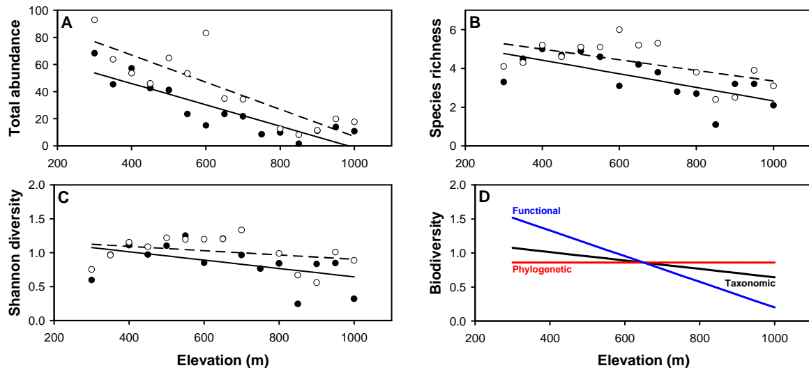
Figure 9 – Empirical relationships (A-C) between elevation and three aspects of mean taxonomic biodiversity of gastropods along two transects (mixed forest and palm forest) in the Luquillo Mountains, as well as hypothesized elevation relationships (D) of taxonomic (black line), functional (blue line), and phylogenetic (red line) biodiversity. Mixed forest transects (solid symbols) and palm forest (open symbols) shown with best fit linear fits.
