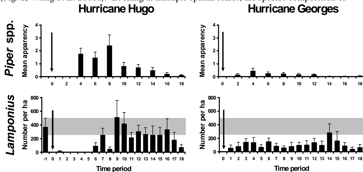
Figure 2 – Effects of repeated hurricanes on abundance of an early successional plant ( Piper spp.) and keystone, herbivorous walking stick ( Lamponius portoricensis ). Each time period is a 6-month interval with hurricanes at time = 0 (arrow). Vertical bars are one ( Piper ) or two ( Lamponius ) SE. Walking sticks exhibited differences in resistance and resilience to the two pulse disturbances, with a new and lower stable state for density following Hurricane Georges. (Willig et al. 2011)
