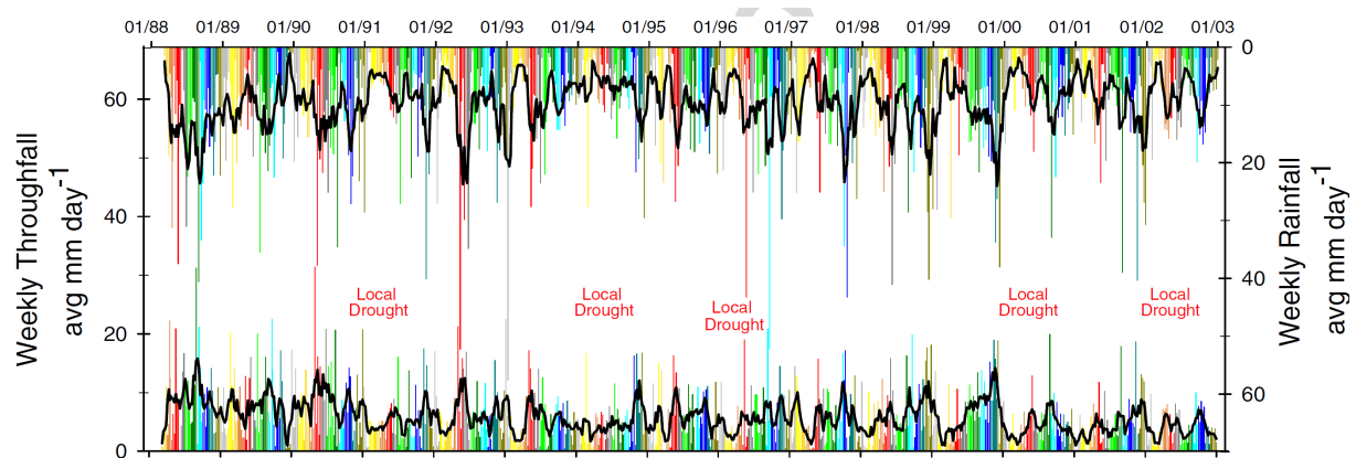
Figure 11 – Throughfall (bottom) and rainfall (top) with periods of local drought indicated (lowest 5% mm d -1 ). Individual colored bars are weekly values coded by month (red is May). Thick black line is running average. (Heartsill-Scalley et al. 2007)
