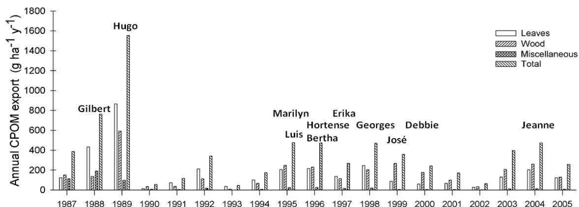
Figure 10 – Long-term annual exports of coarse particulate organic matter (CPOM) from the Bisley Experimental Watersheds. The names over the bars refer to tropical storms or hurricanes that affected the area. Peak CPOM exports correspond to major hurricanes (e.g., Hurricane Hugo in 1989), but periods of frequent storm activity (e.g., 1995-2000) can result in low but continuous exports. (Re-drawn from Heartsill-Scalley et al. 2012)
